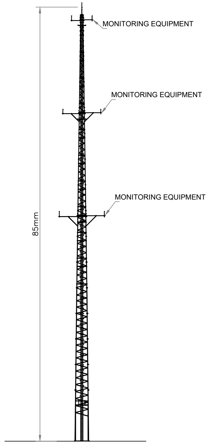
85m LATTICE MAST
